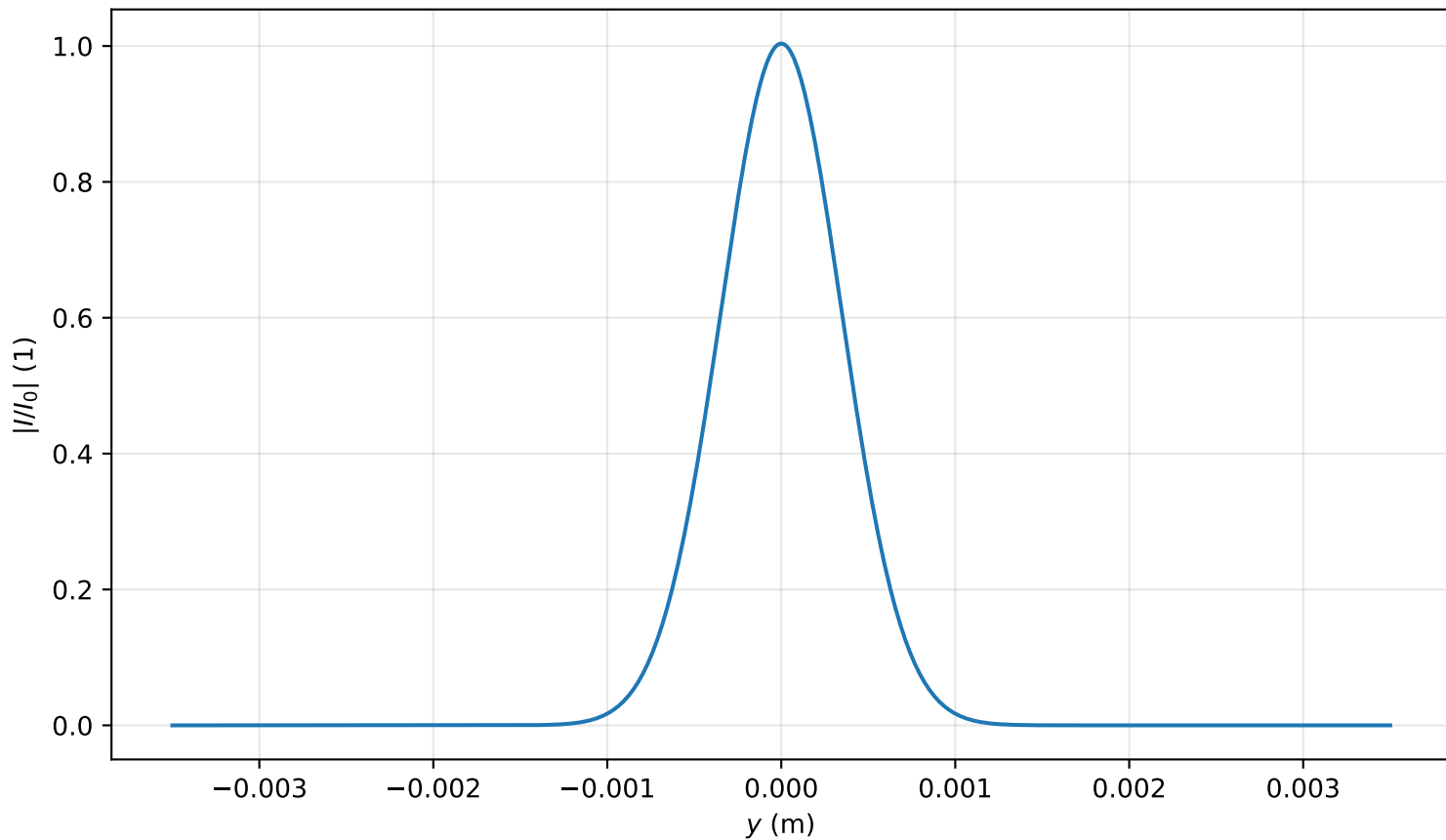
Intensity profile I(x=0, y, z=0.159)/I_0 , P_{in}=0.4P_{cr} , artificial time
